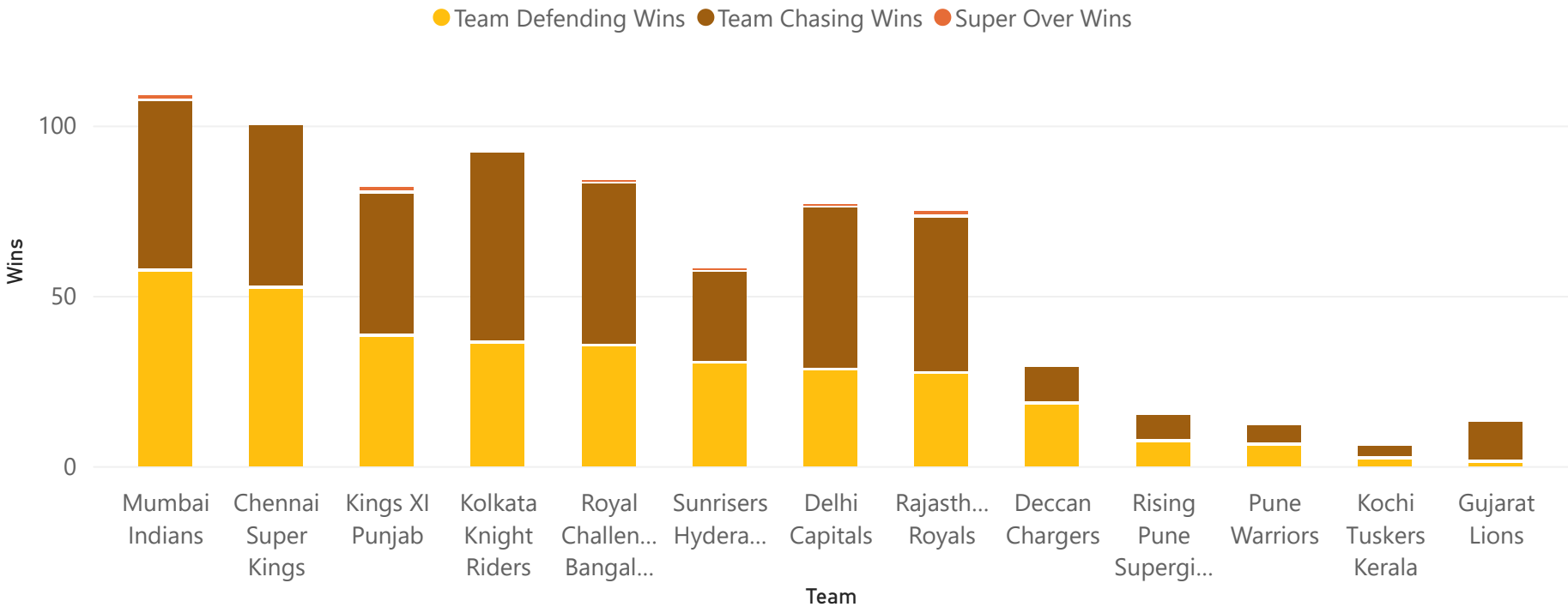
Team Defending Wins, Team Chasing Wins and Super Over Wins by Team
