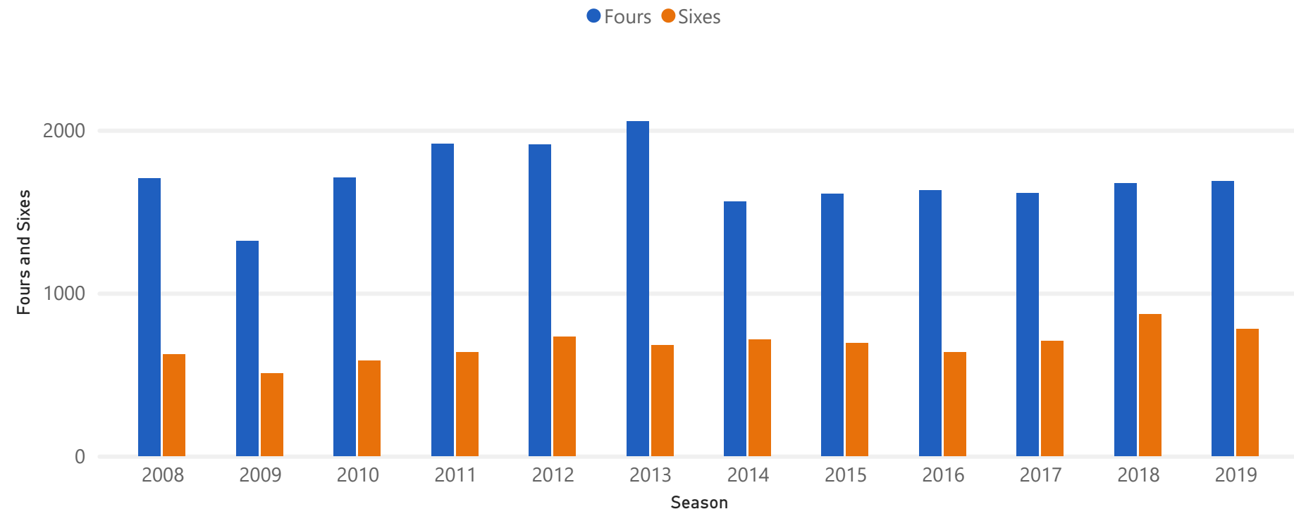
Fours and Sixes by Season
