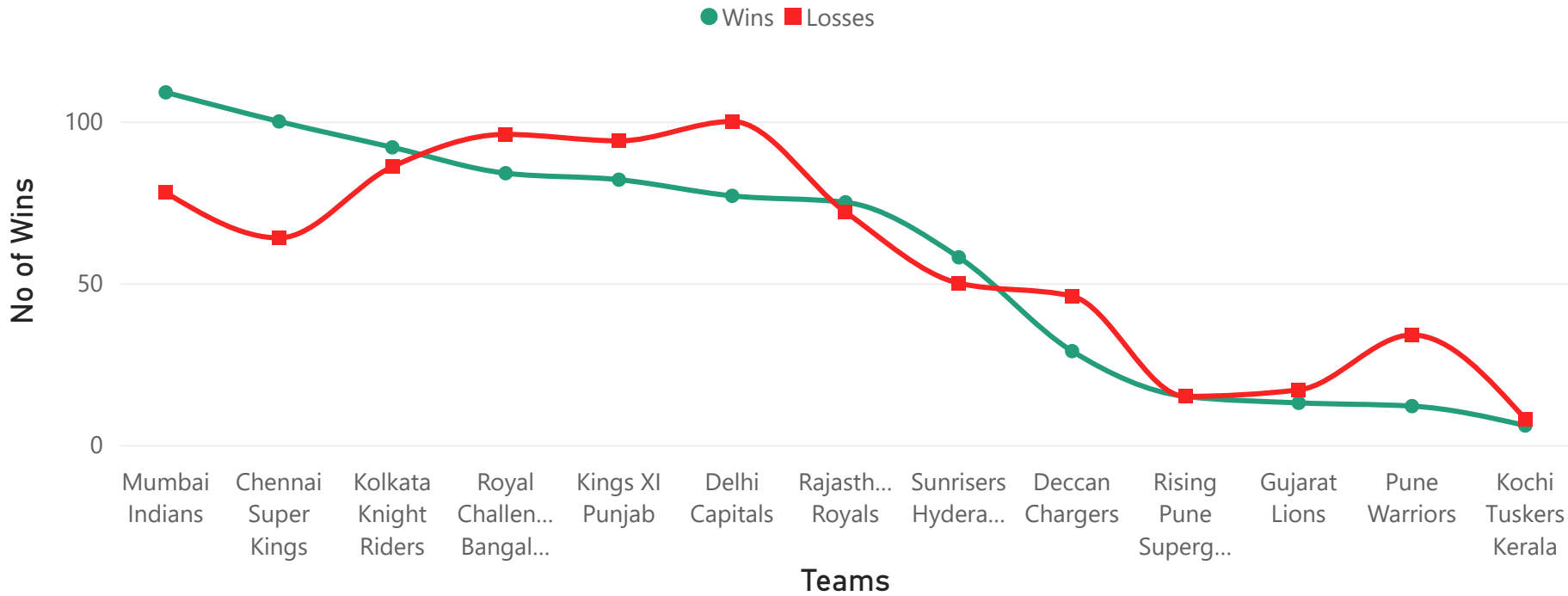
Wins and Losses for each team
