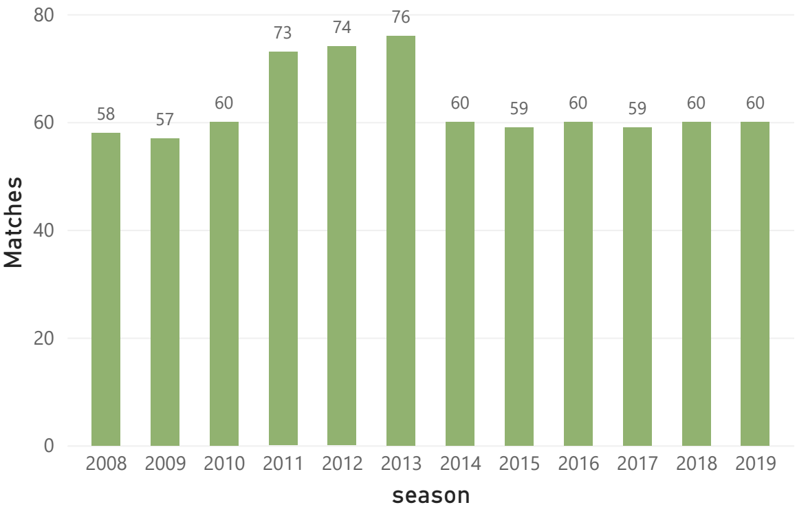
Matches per Season
