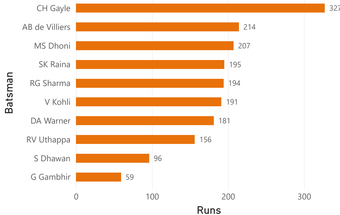
Top 10 Six Hitters
