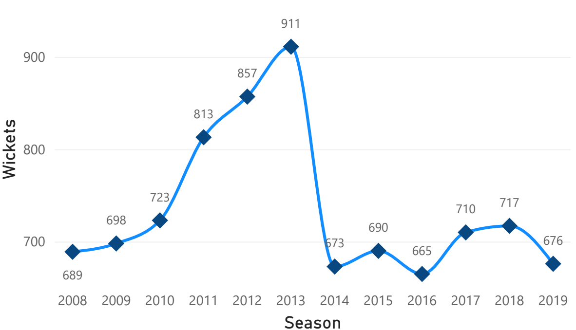
Total wickets per season
